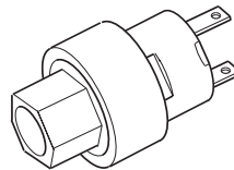
SW-90418 (s/sedes SW-85225) GM CLUTCH CYCLING SWITCH A VARIATION ON THE LOW PRESSURE CUT OUT SWITCH. UNLIKE NORMAL LP SWITCHES, IT IS USUALLY INSTALLED ON THE ACCUMULATOR ON THE LOW SIDE OF THE SYSTEM. CUT-OUT: 27 psi CUT-IN: 35 psi REPLACES OEM 3041409 AND 3041596
