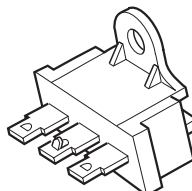
SW-83250 THERMAL LIMITER FUSE USED ON SOME DELCO SYSTEMS WITH SUPERHEAT SWITCHES.
